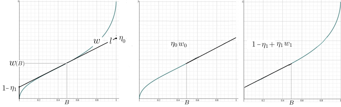
Figure 1: Decomposition of the inverse S -shaped distortion function w of (29) with parameter r = 0.61 and inflection point B \approx 0.48 . The linear function l is used to construct distortions w_0 and w_1 in (30).
